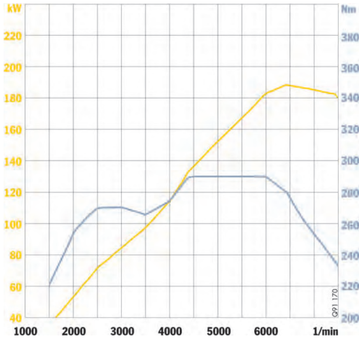
Boxster power/torque diagram
